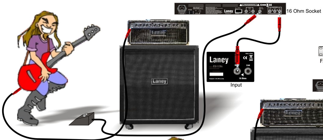
System using 1* LH50 Head 1* GS4121A
